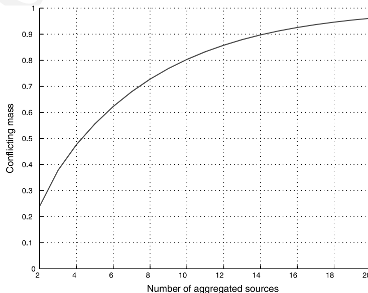
Fig. 1. Conflict vs. number of sources to combine.
